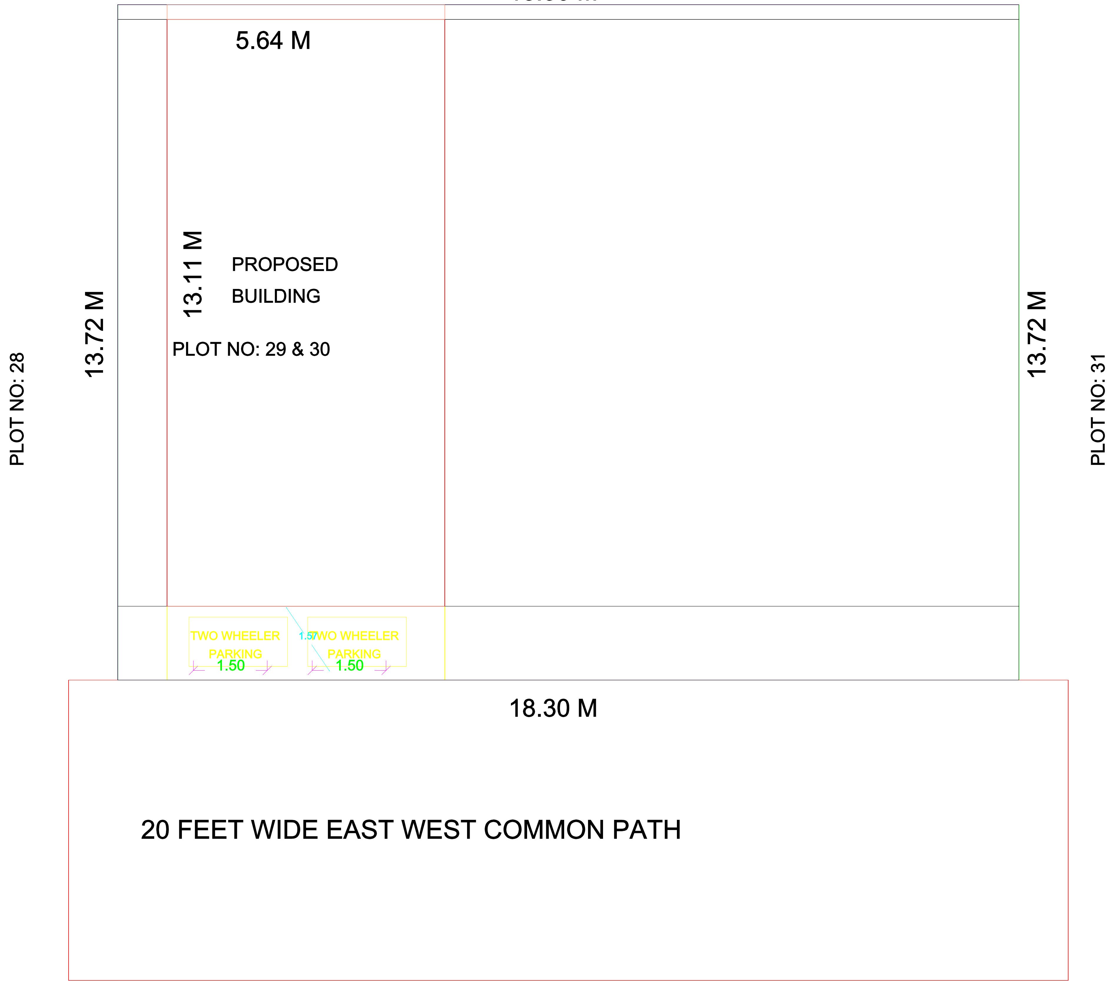
SITE PLAN
