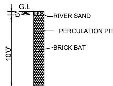
PERCULATION PIT
