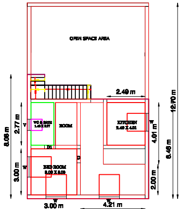
PROPOSED FIRST FLOOR PLAN (EXTENSION)
