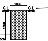
SECTION OF PEBBLE TRENCH
