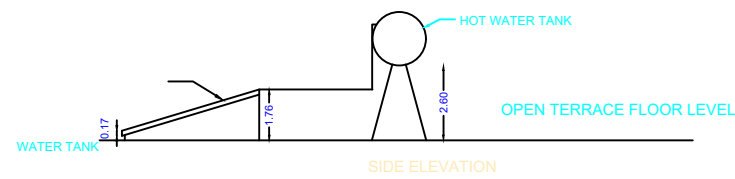
SIDE ELEVATION
