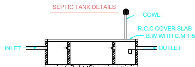
SECTIONAL ELEVATION
