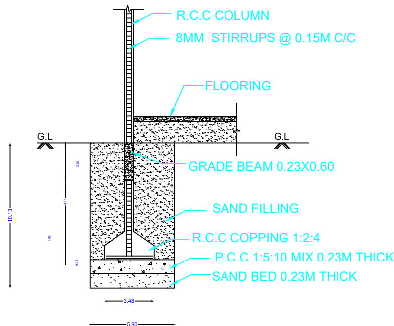
FOUNDATION DETAILS
