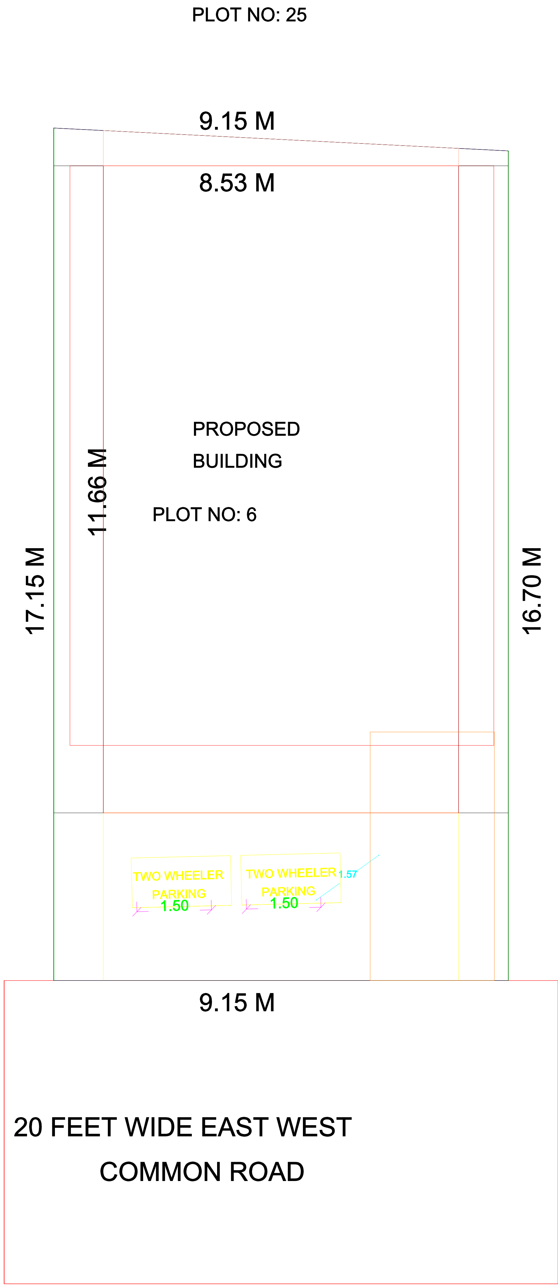
SITE PLAN
