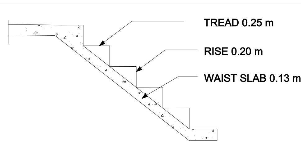
STAIR DETAILS
