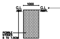
SECTION OF PEBBLE TRENCH SCALE : 1 : 100
