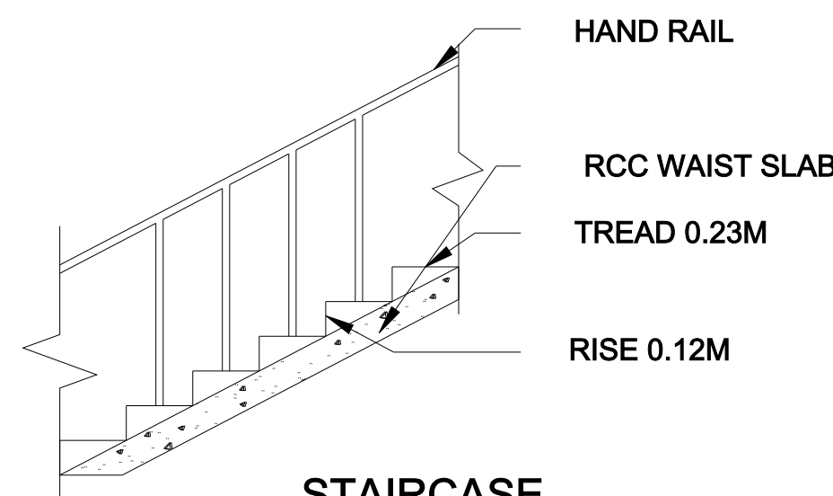
STAIRCASE
