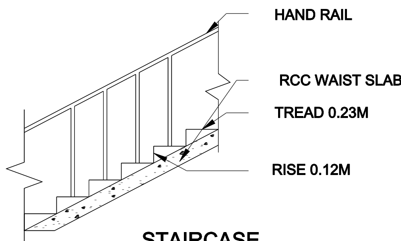
STAIRCASE
