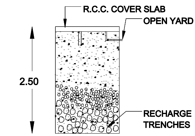
SECTION C-C'
