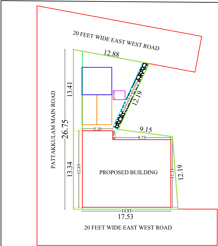
SITE PLAN
