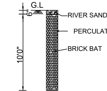
PERCULATION PIT
