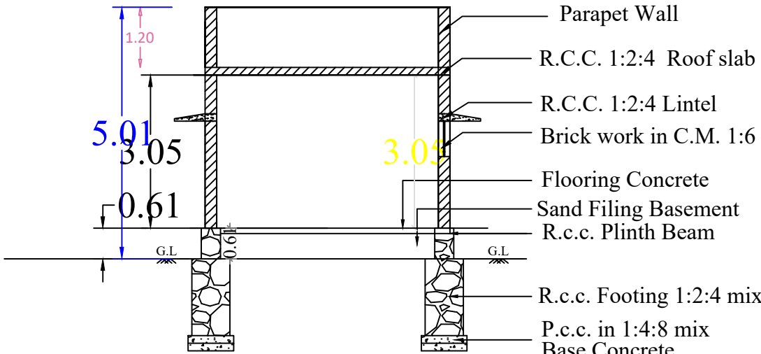
SECTION -"AB"
