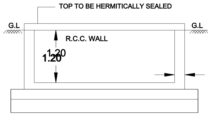
RWH SECTION
