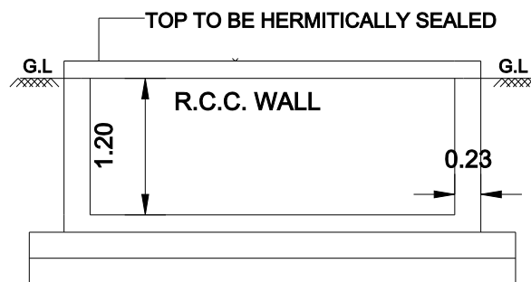
RWI SECTION ( SAMPLE )
