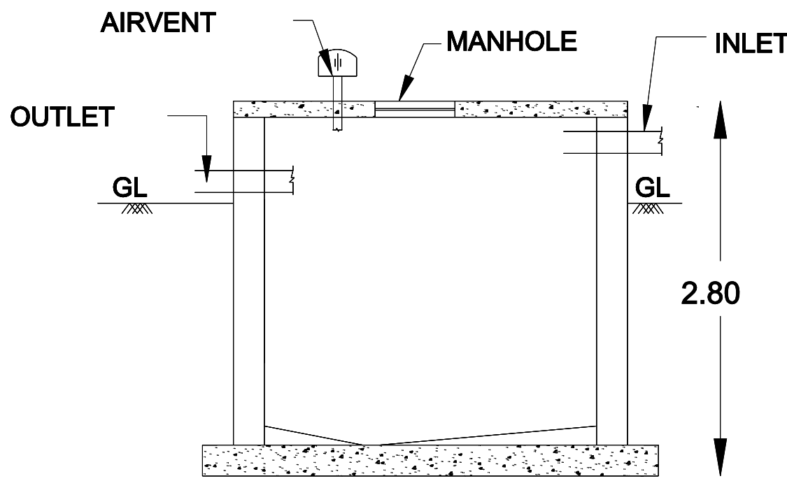
SECTION B-B'
