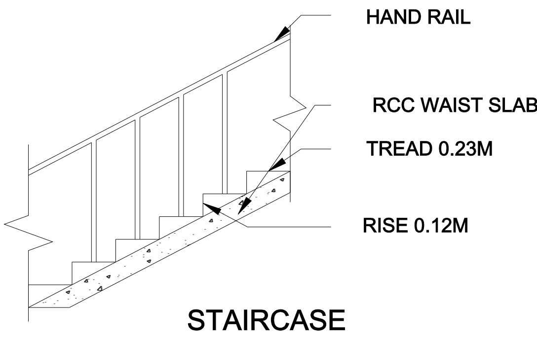
STAIRCASE
