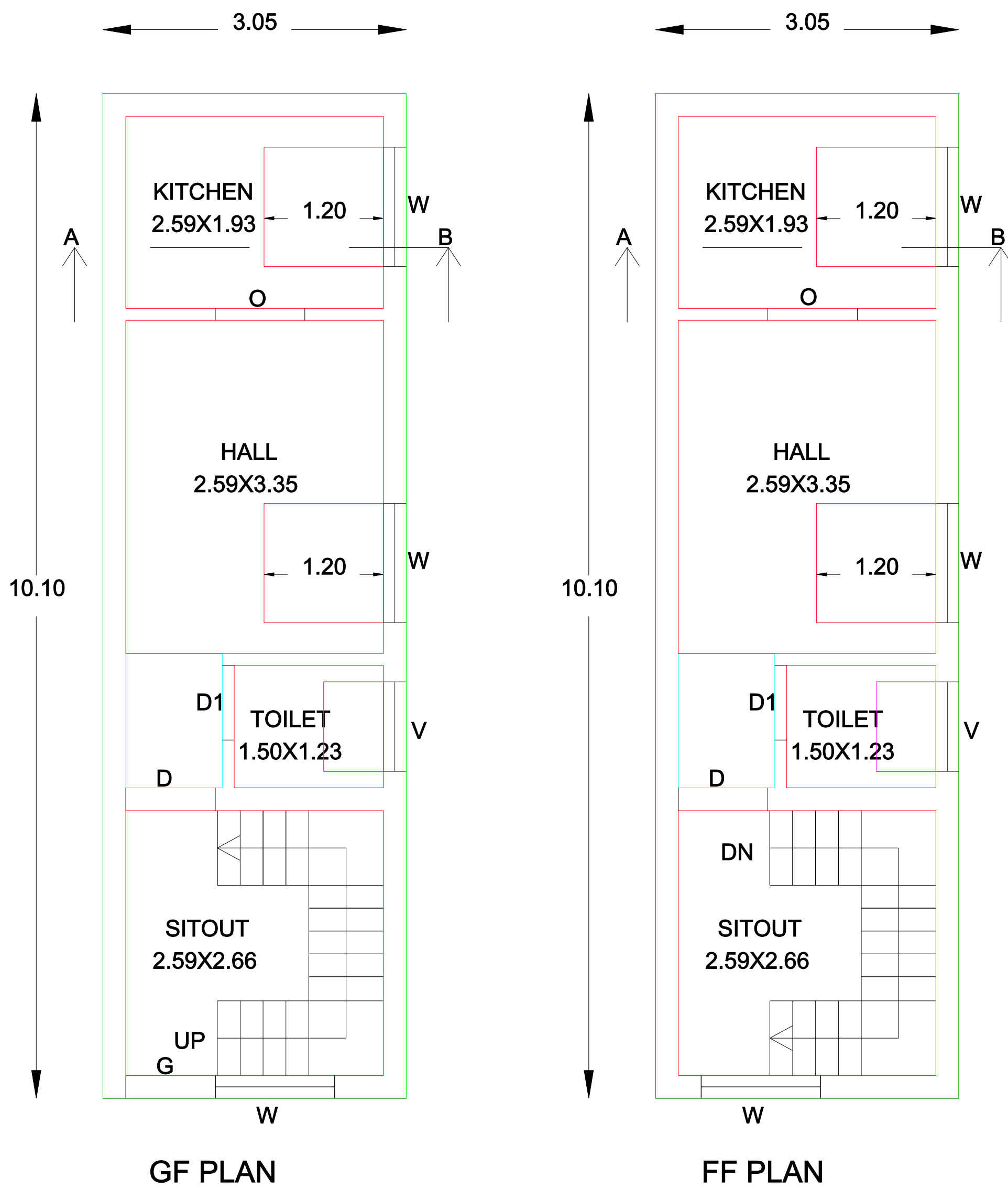
GF PLAN
