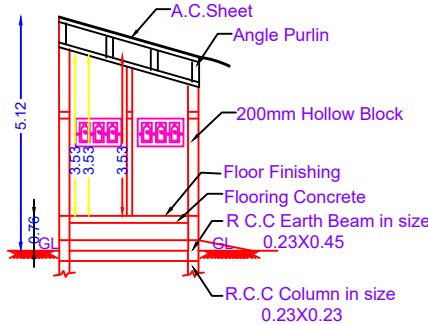
SECTION ON "PQ" SCALE 1:100
