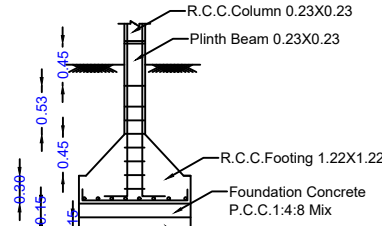
DETAILS OF COLUMN FOOTING (SCALE 1:50)
