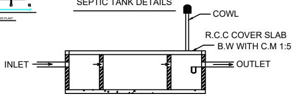
SECTIONAL ELEVATION
