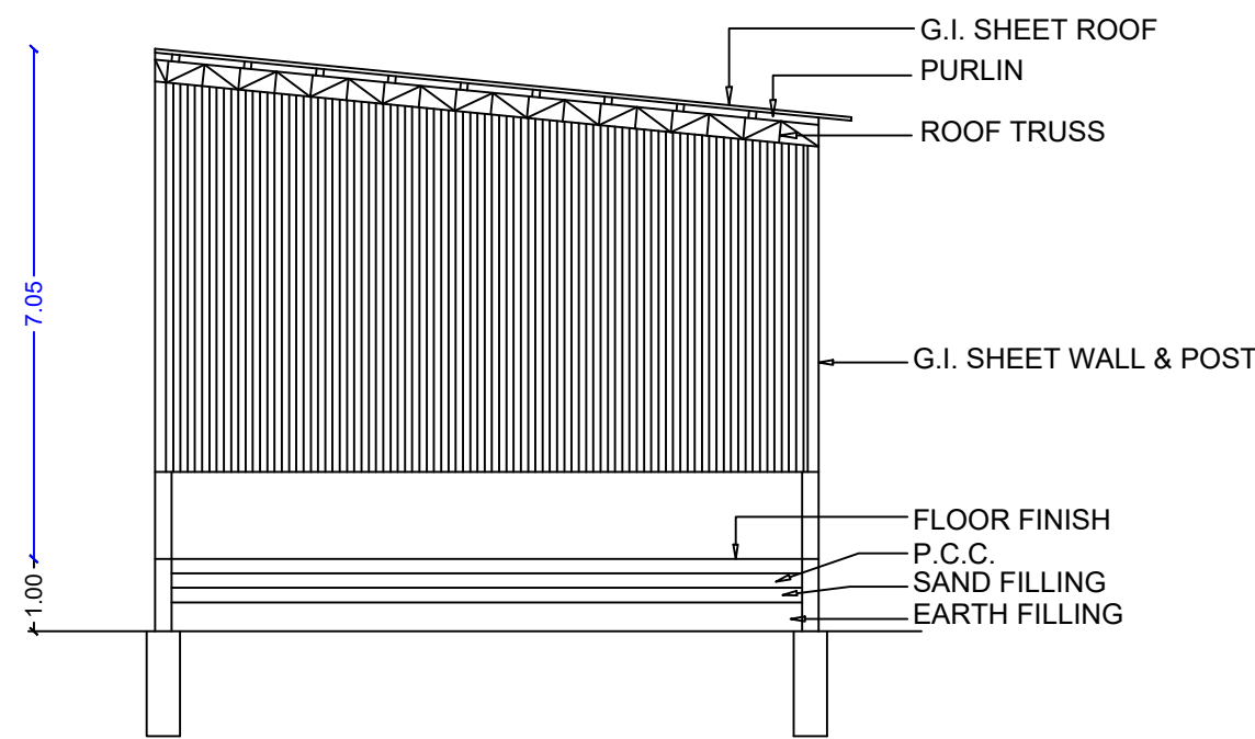
SECTION ON "XY"
