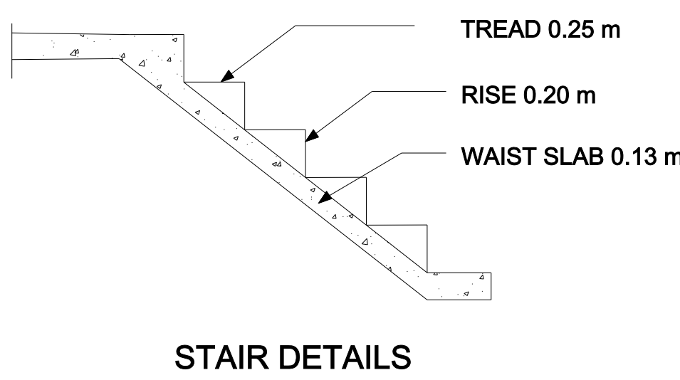
STAIR DETAILS
