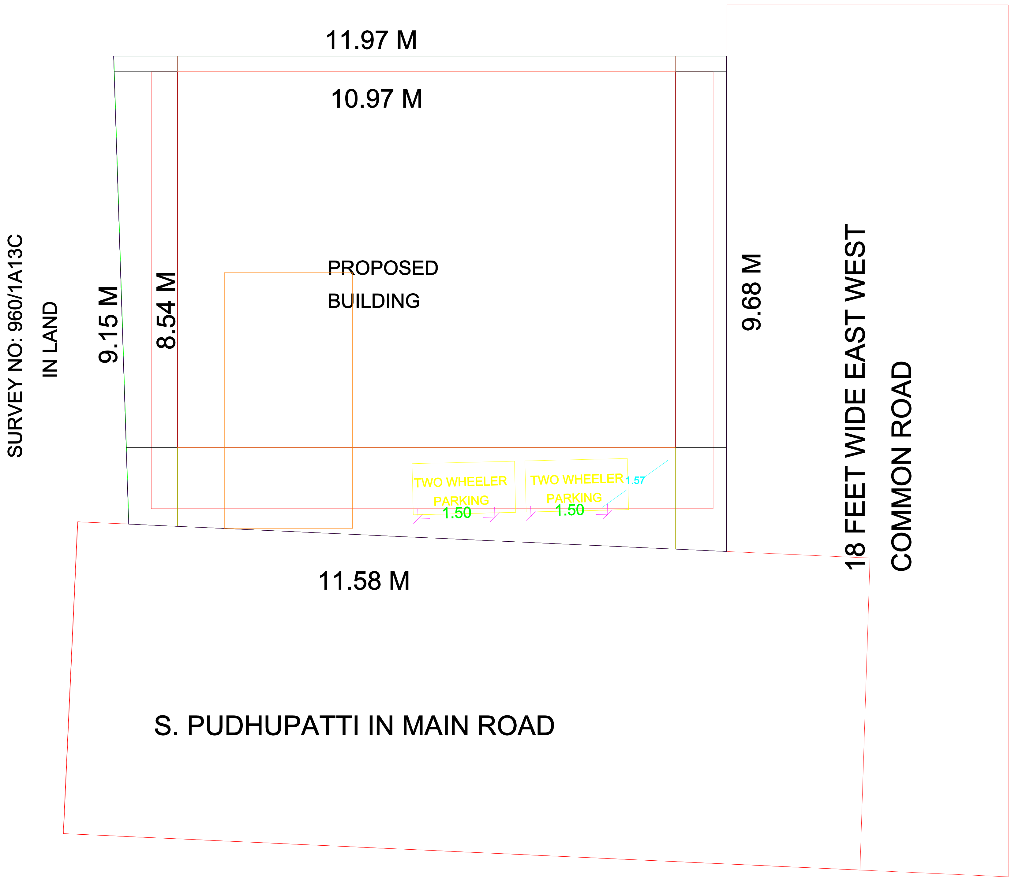
SITE PLAN
