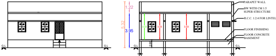
FRONT ELEVATION
