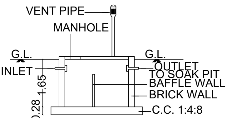
SECTION OF SEPT. TANK
