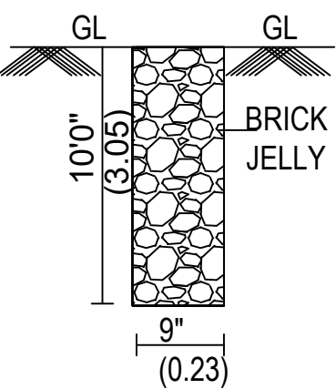
PERCOLATION PIT:-
