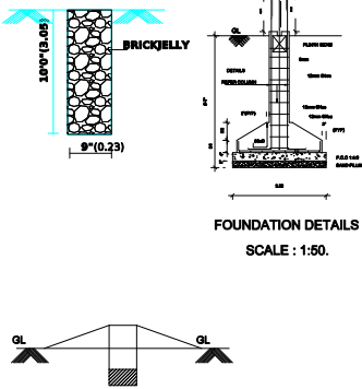
Dwarf Wall Details
