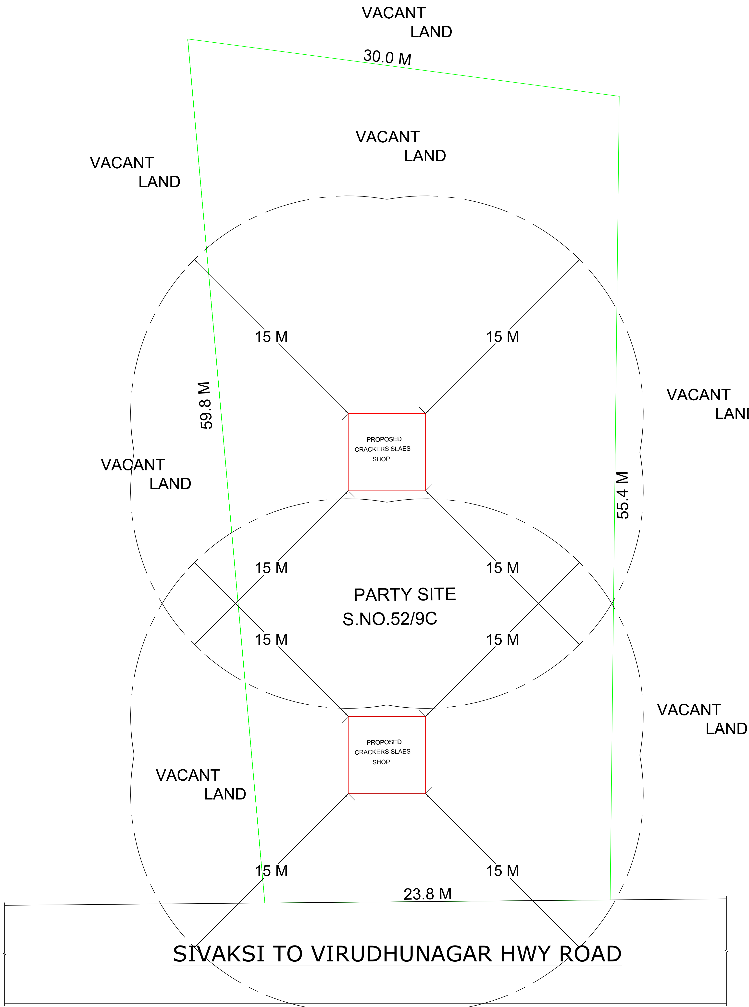
SITE PLAN
