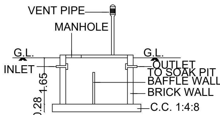
SECTION OF SEP.TANK
