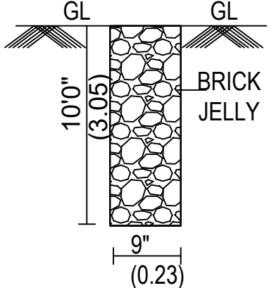
PERCOLATION PIT:-
