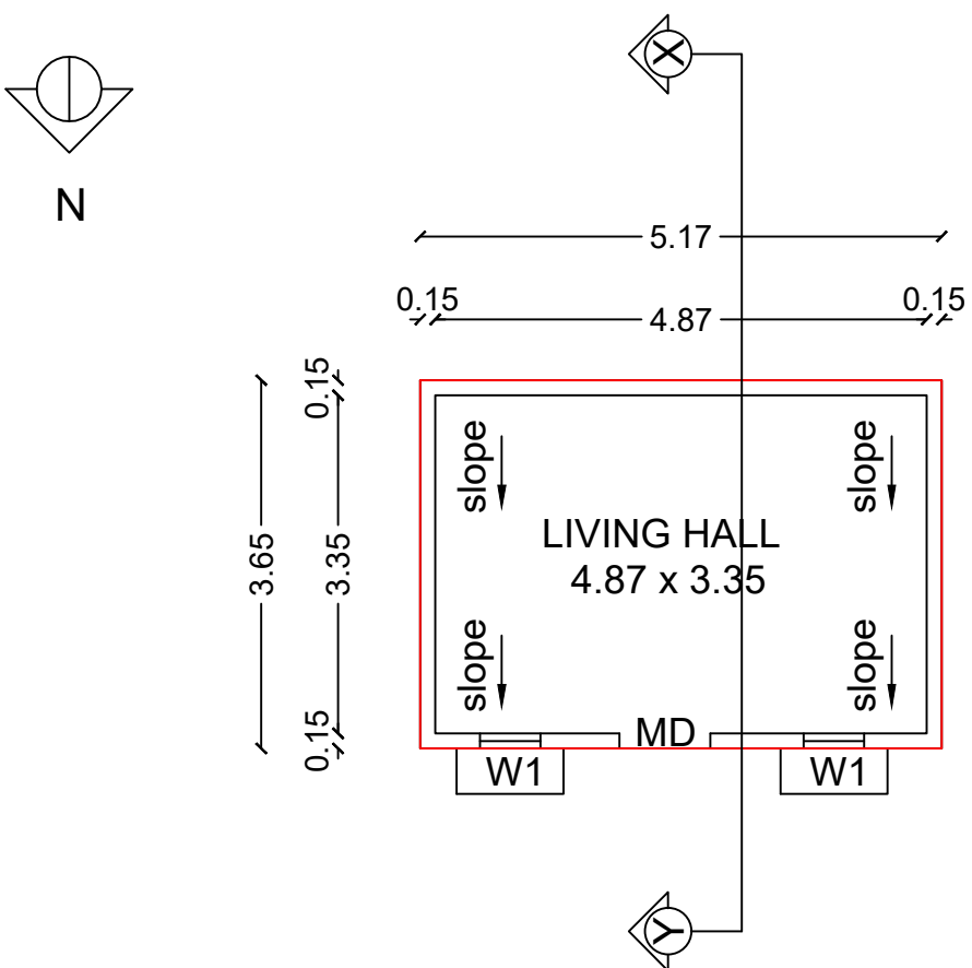
PROPOSED GROUND FLOOR PLAN ( ASBESTOS SHEET ROOF )
