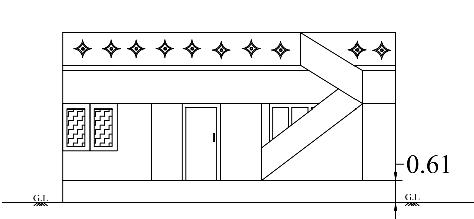
FRONT ELEVATION
