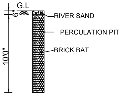
PERCULATION PIT
