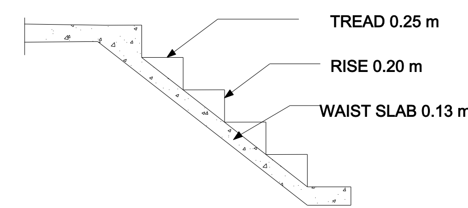
STAIR DETAILS
