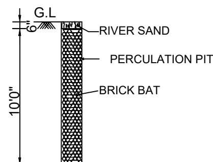
PERCOLATION PIT
