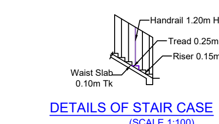
DETAILS OF STAIR CASE (SCALE 1:100)
