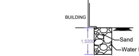
DETAILS OF RAIN PERCOLATION (SCALE 1:100)
