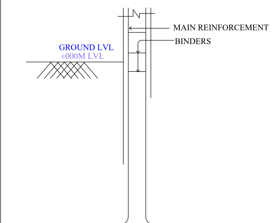
SECTION ON D-D
