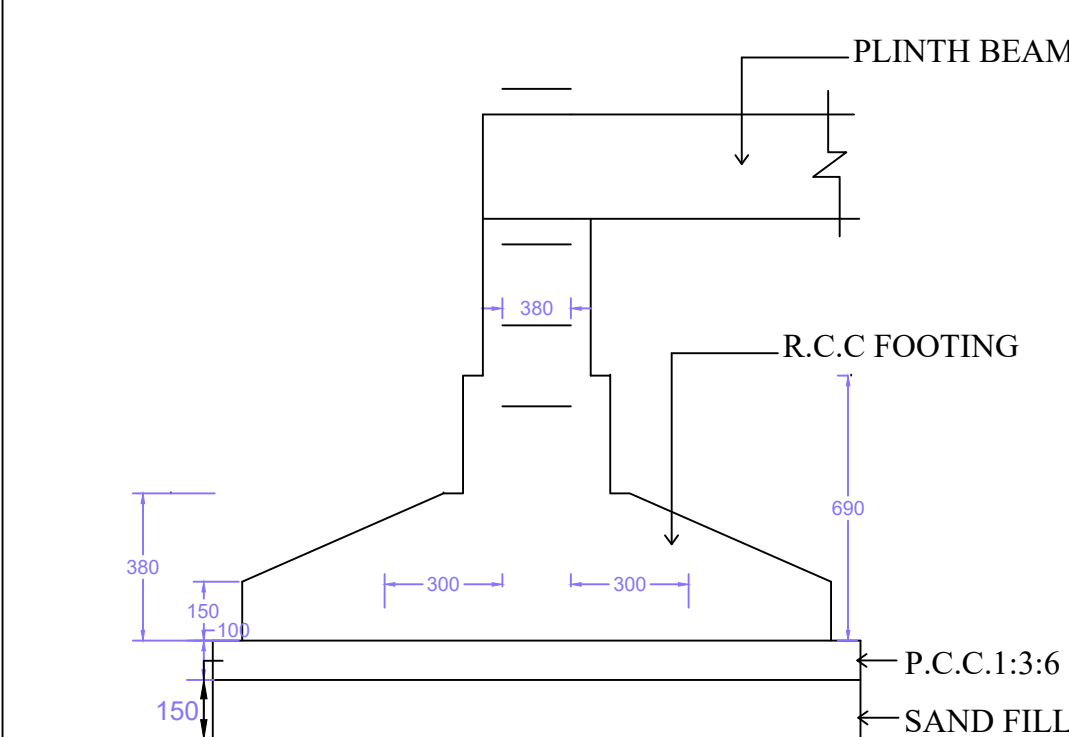
TYPICAL SECTION OF R.C.C COLUMN FOUNDATION SCALE : 1" = 2'-0"
