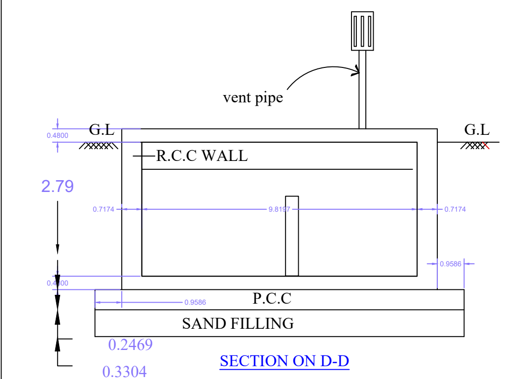
SECTION ON D-D
