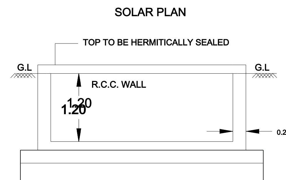
RWH_CAPACITY_L = 2000 RWH SECTION
