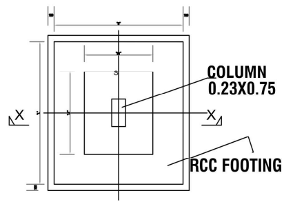
TYP. PLAN OF FOOTING SCALE - 1:75
