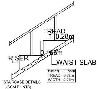
STAIRCASE DETAIL
