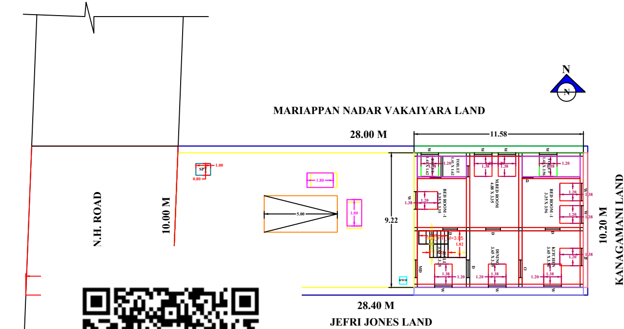
SITE & GROUND FLOOR PLAN
