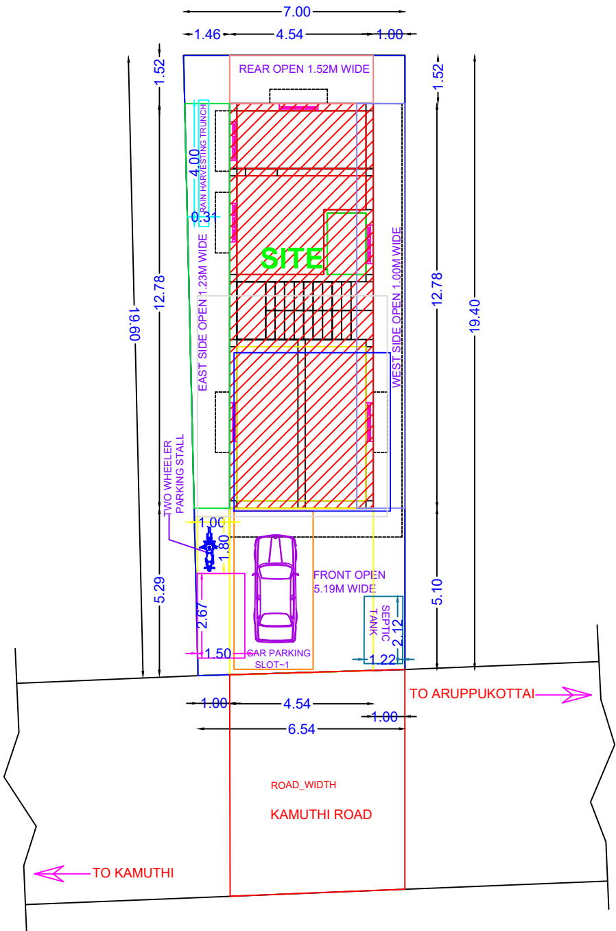
SITE PLAN
