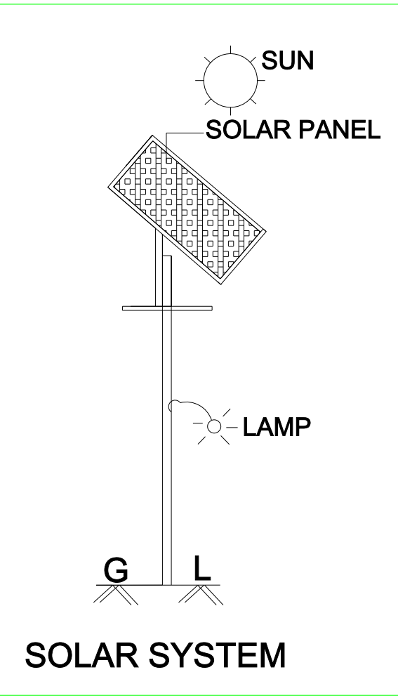
SOLAR SYSTEM
