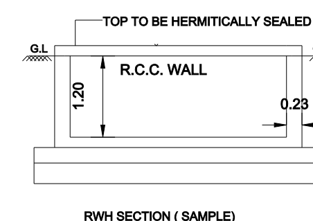
RWY SECTION / SAMPLE
