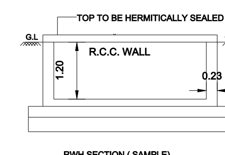
RWY SECTION / SAMPLE
