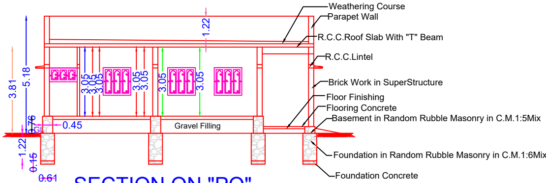
SECTION ON "PQ" SCALE 1:100
