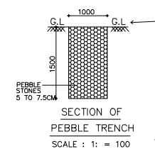
RWH_SECTION (SAMPLE) RWH_CAPACITY_L = 2000LTRS
