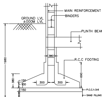
C.C COLUMN FOUNDATION
