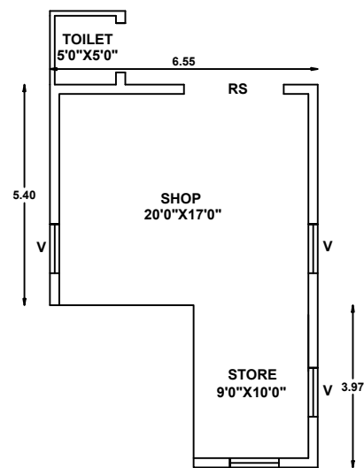
PROPOSAL GROUND FLOOR PLAN
