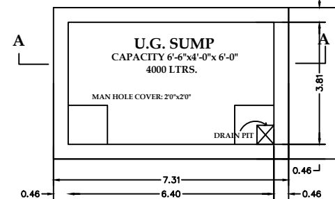
SUMP DETAIL SCALE 1"=4'0"
