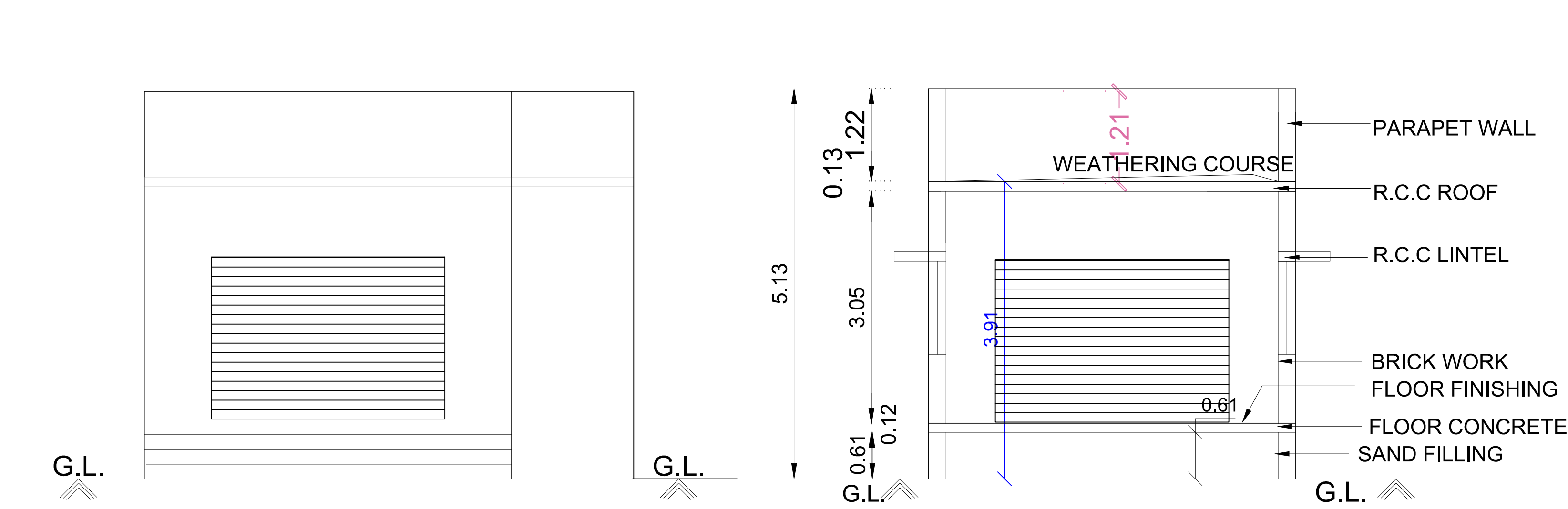
FRONT ELEVATION
