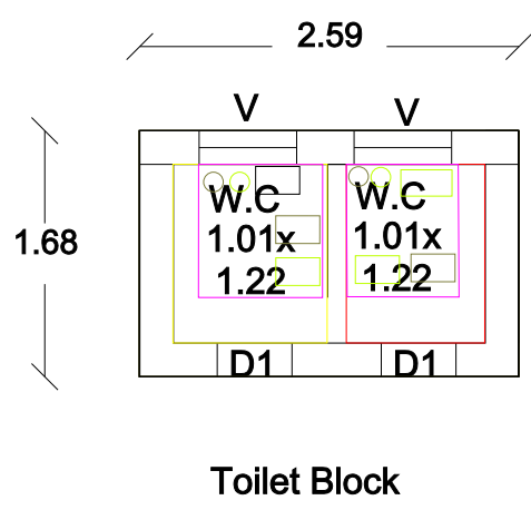
Toilet Block
