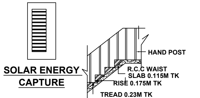
DETAILS OF STAIRCASE
