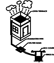
RAIN WATER SAVINGS ARRANGEMENTS
