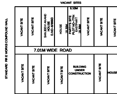
SITE PLAN SCALE:1CM=4M
