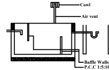
SEPTIC TANK - SECTION
