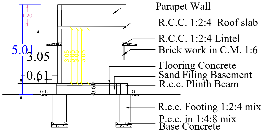
SECTION -"AB"
