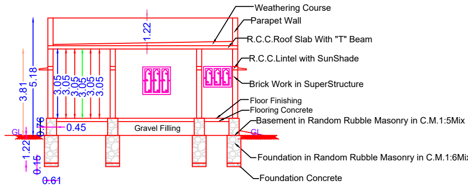
SECTION ON "PQ" (SCALE 1:100)
