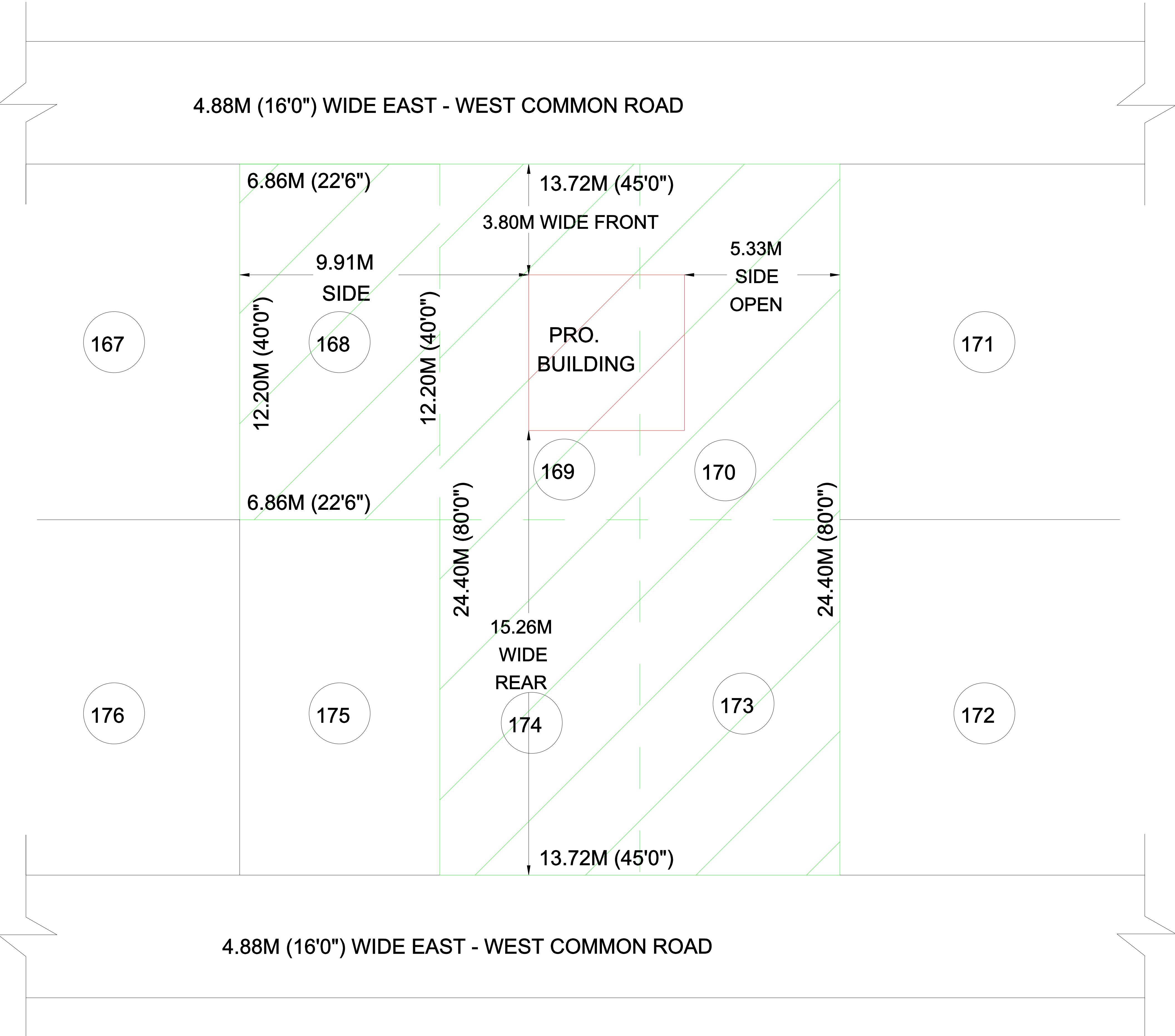
LOCATION PLAN
