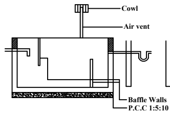
SEPTIC TANK - SECTION
