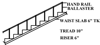
STAIRCASE
