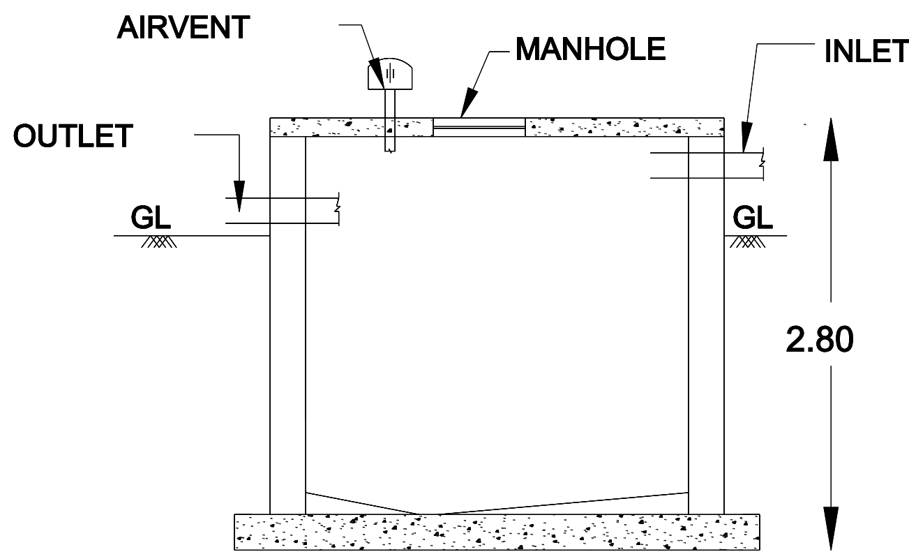
SECTION B-B'
