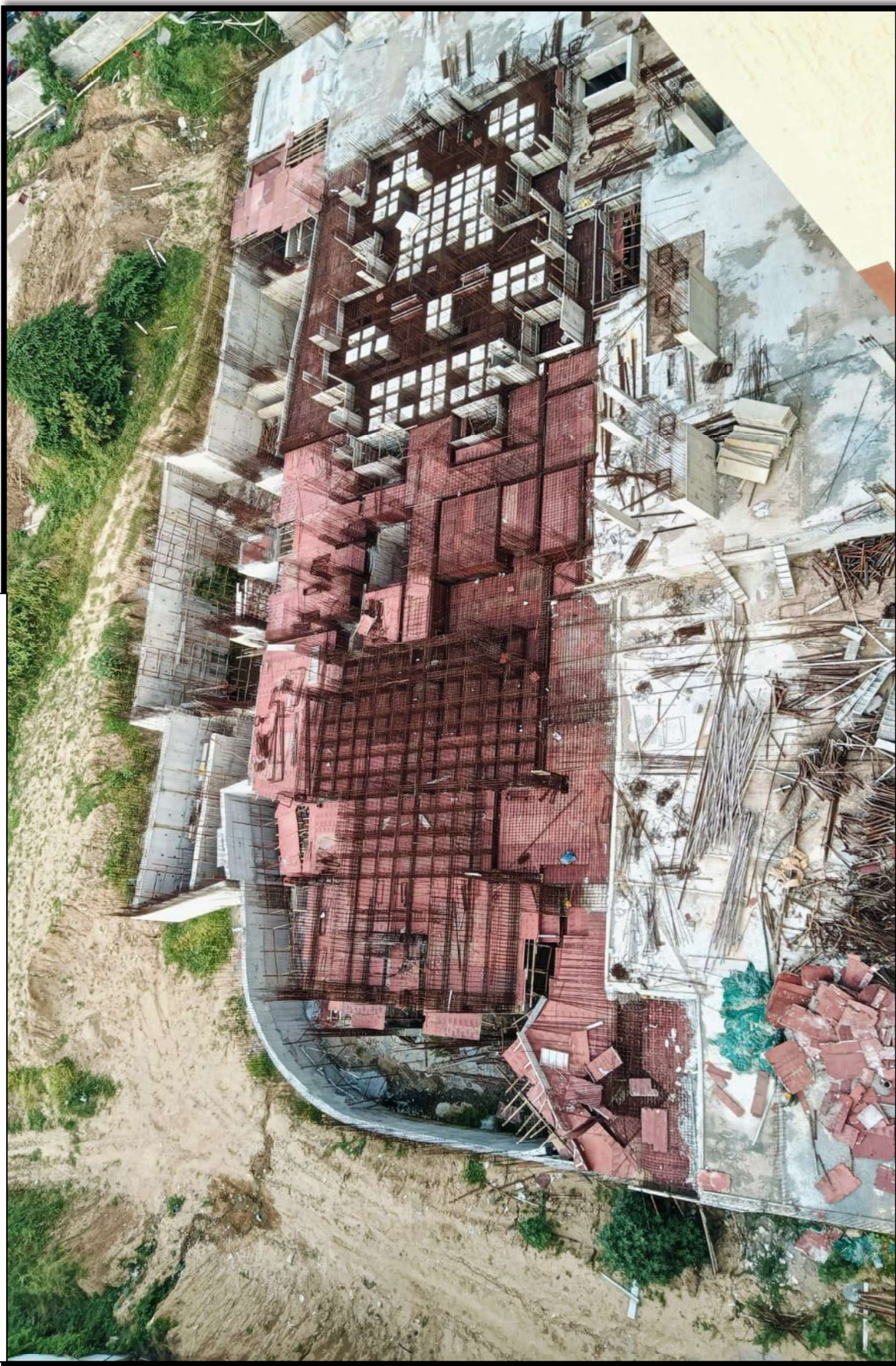
Tower 4B Void slab & R Wall work in progress
