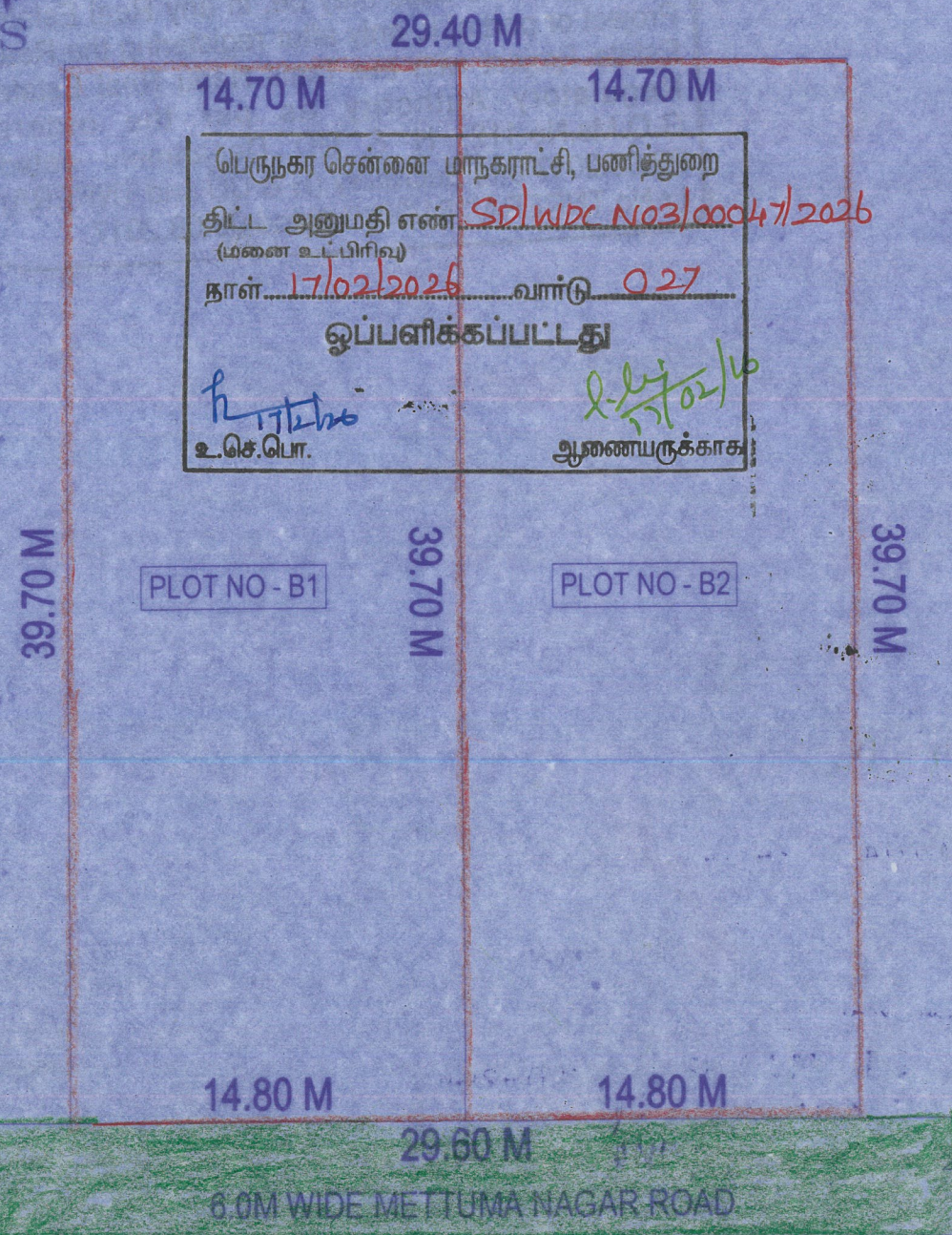
PROPOSED SUB-DIVISION PLAN SCALE - 1 : 200
